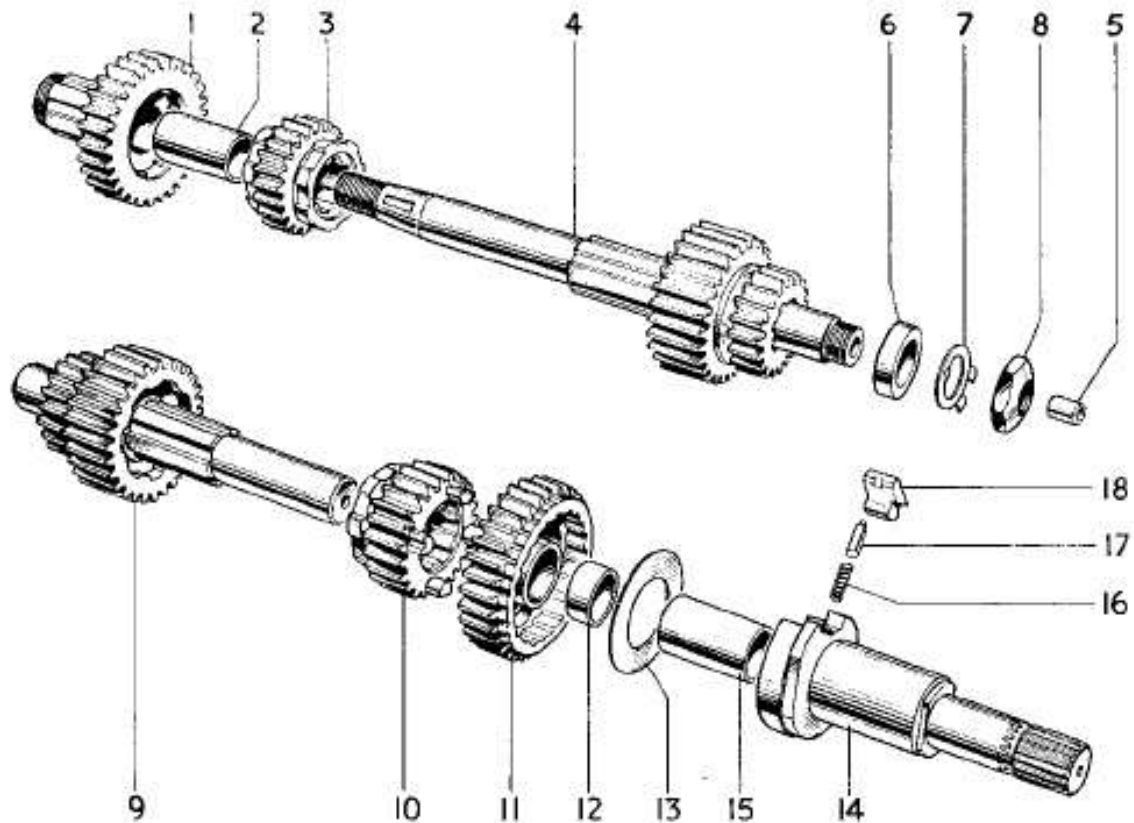
FIG. 6 SHAFTS AND GEARS
