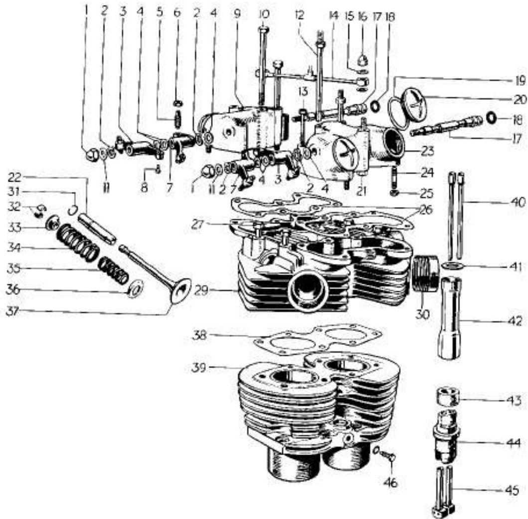
FIG. 3 CYLINDER BLOCK AND HEAD, 5TA INDEX TO FIG. 3
