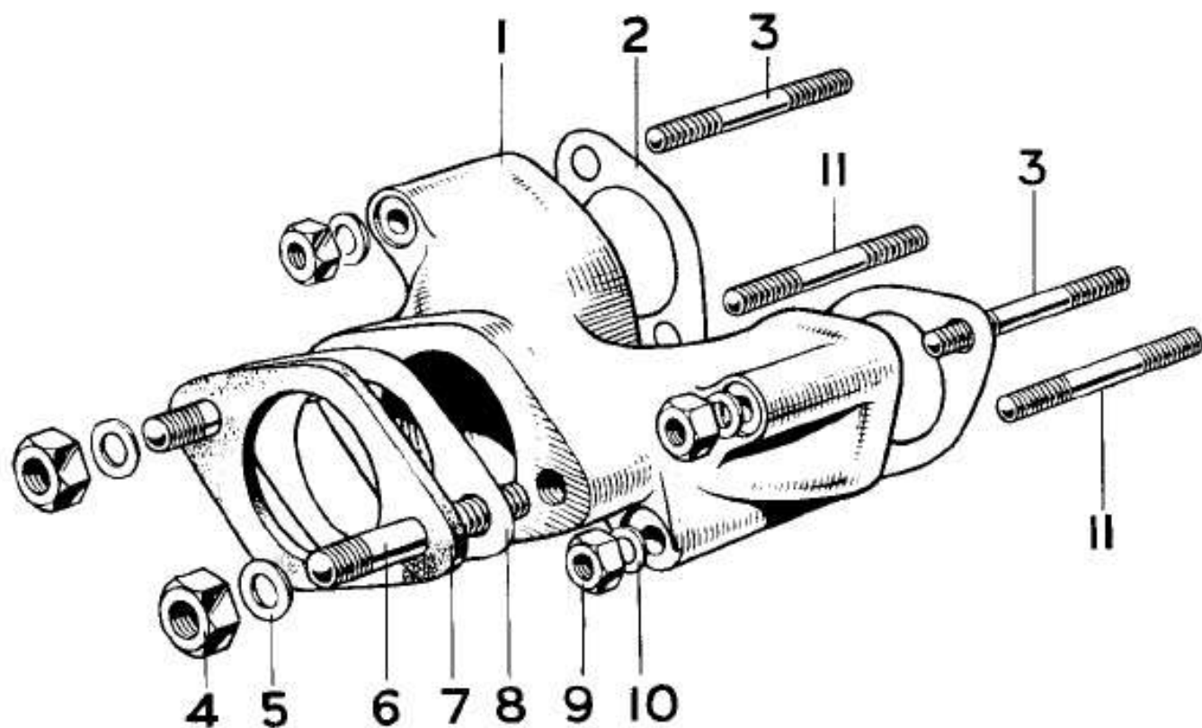
FIG. 1 INLET MANIFOLD
