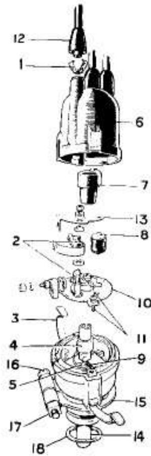
FIG. 20 LUCAS DISTRIBUTOR TYPE 18D2
