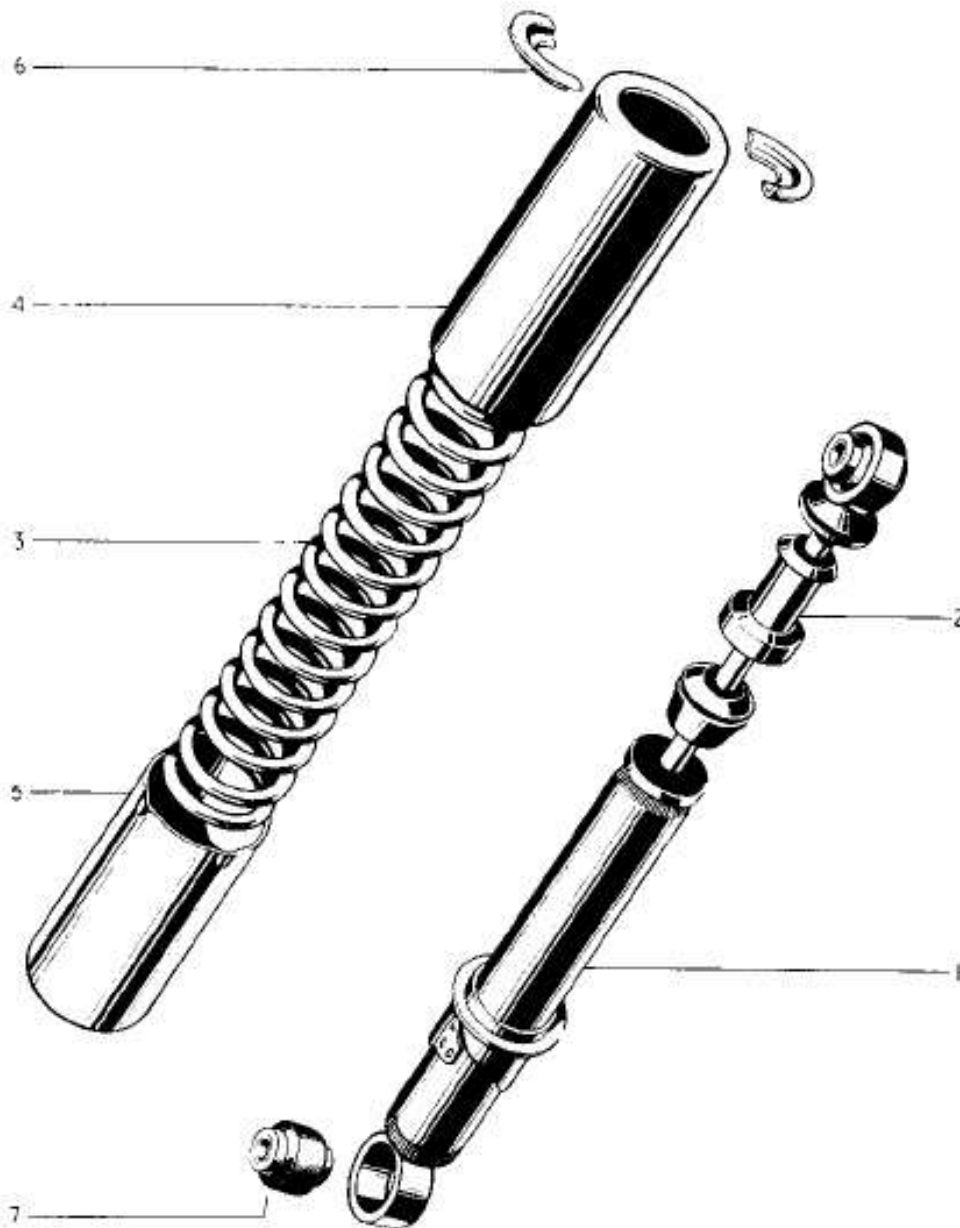
FIG. 22 GIRLING SUSPENSION UNIT
