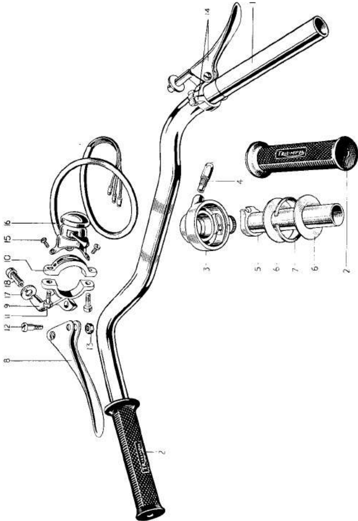
FIG. 18 HANDLEBAR AND CONTROLS
