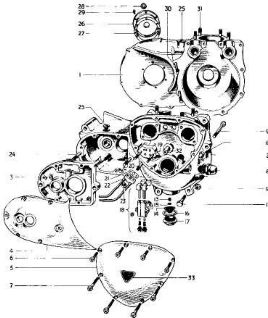
FIG. 5 CRANKCASE AND COVERS
