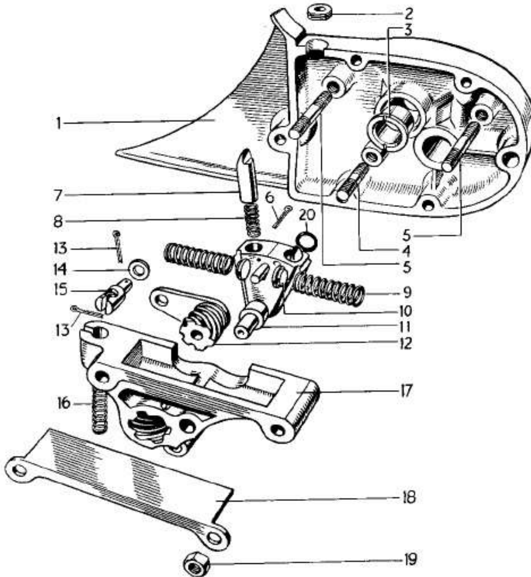
FIG. 8 GEARBOX OUTER COVER
