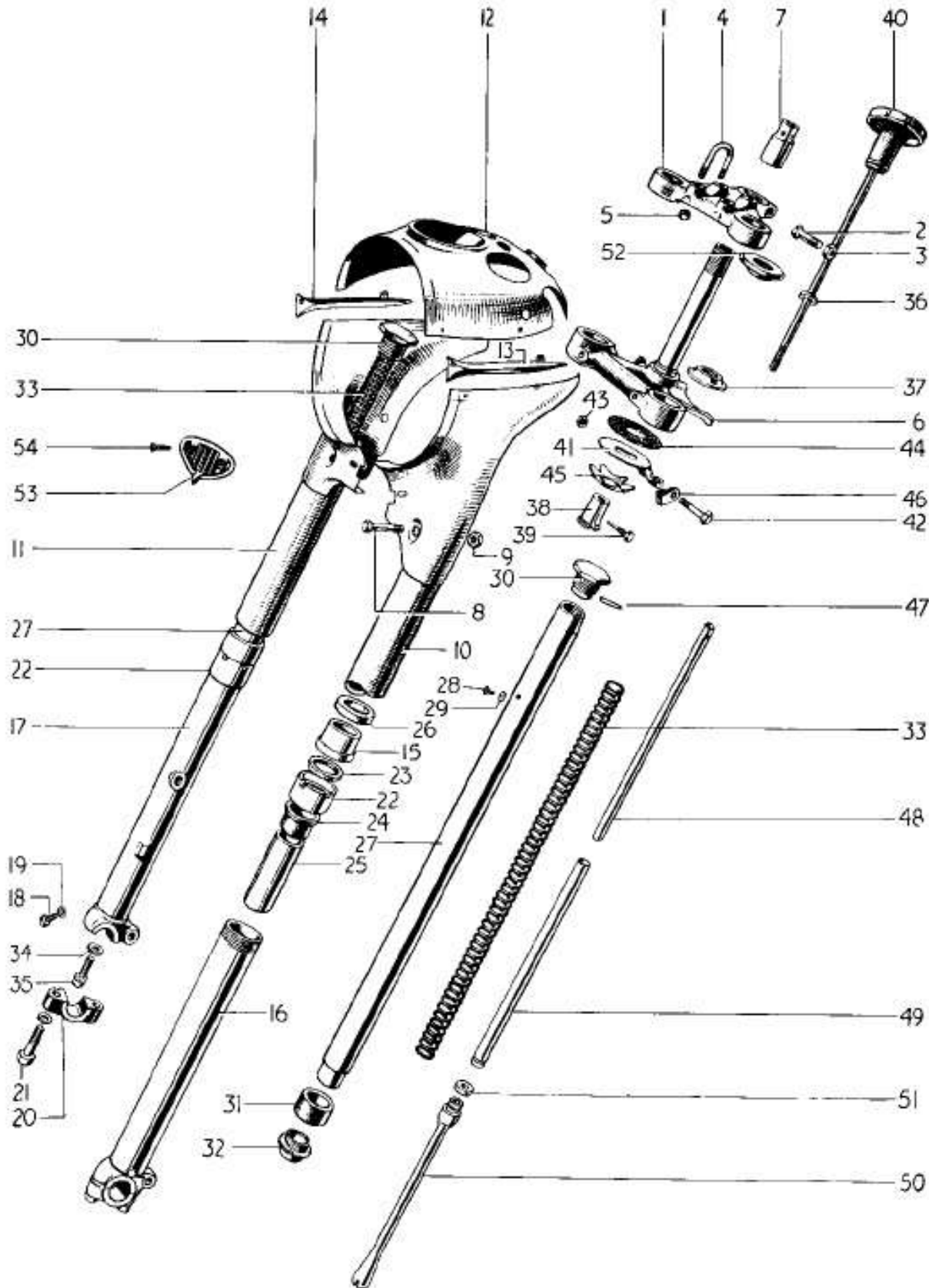
FIG. 11 TELESCOPIC FRONT FORK
