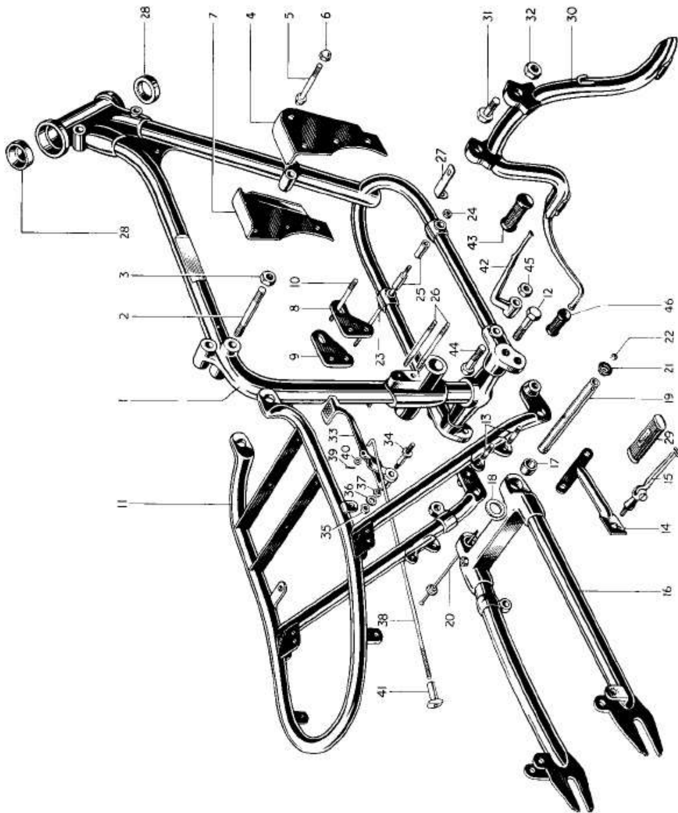
FIG. 10 FRAME AND FITTINGS
