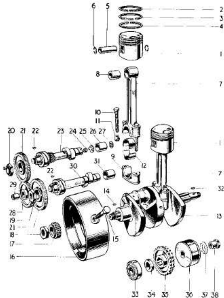
FIG. 4 CRANKSHAFT AND CONNECTING RODS INDEX TO FIG. 4
