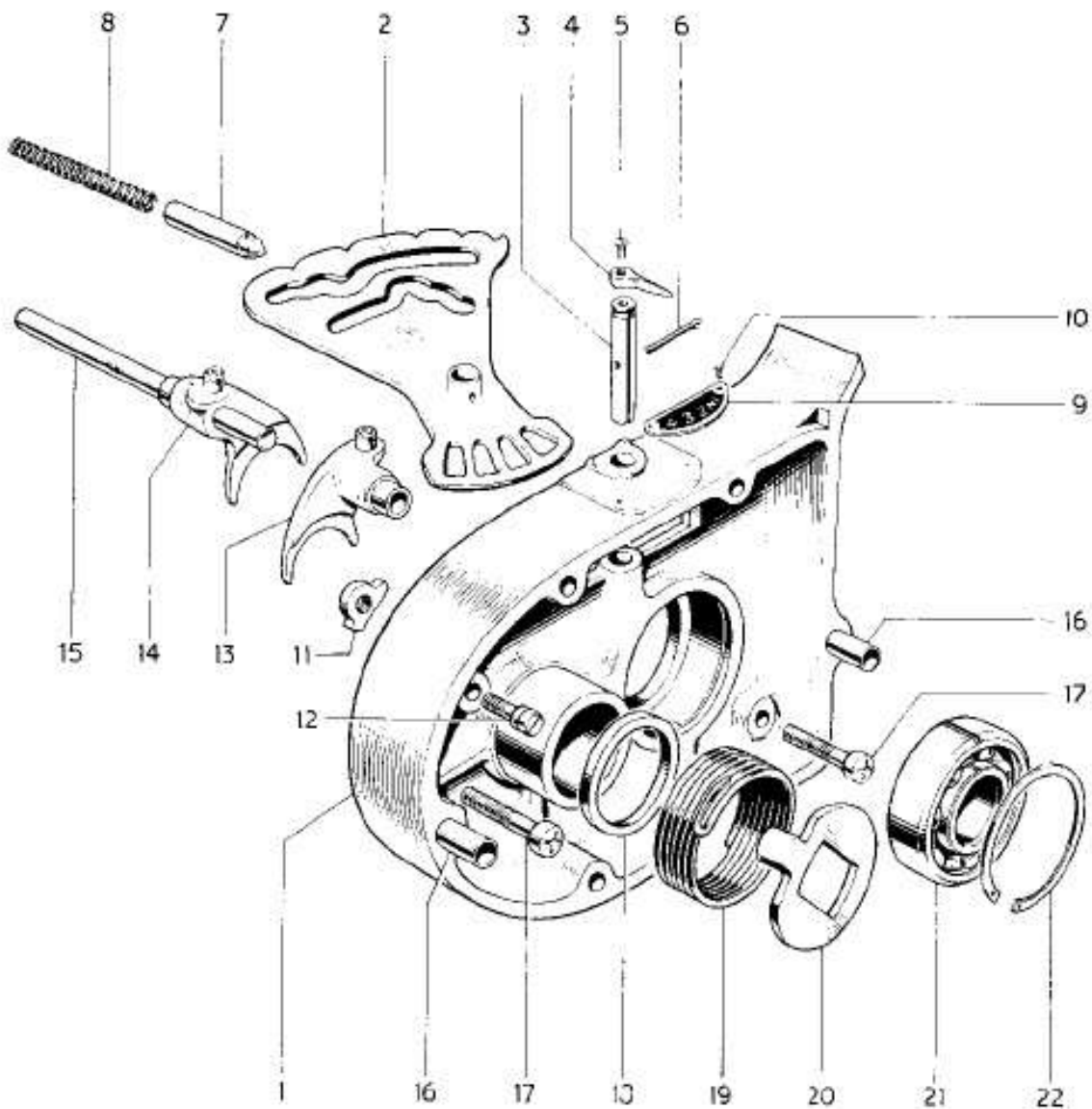
FIG. 7 GEARBOX INNER COVER
