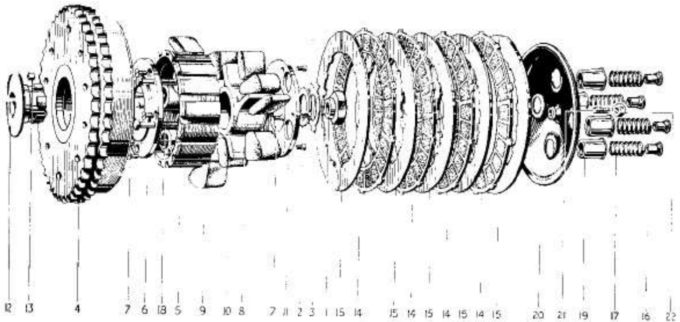
FIG. 9 CLUTCH AND SHOCK ABSORBER
