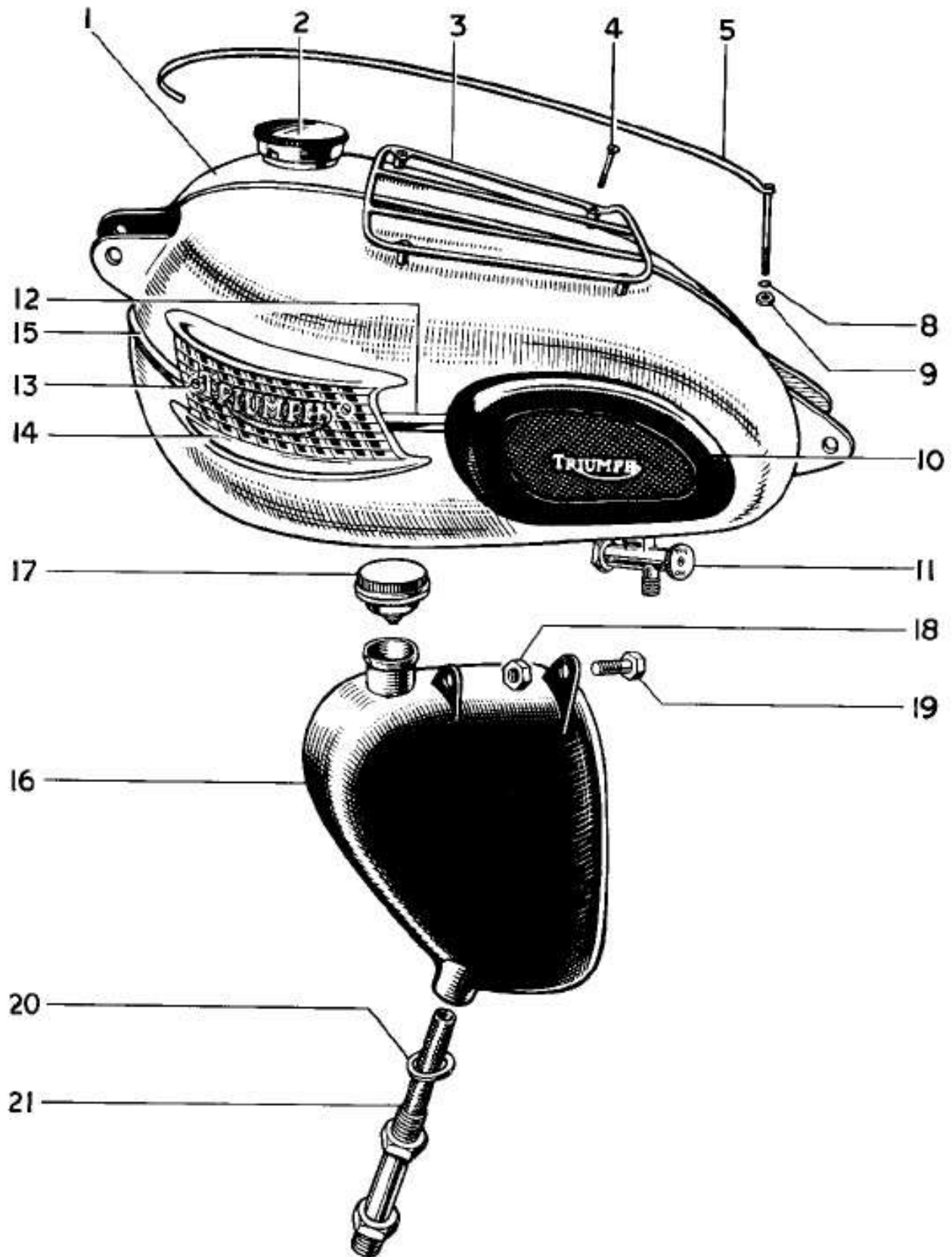
FIG. 15 PETROL AND OIL TANKS
