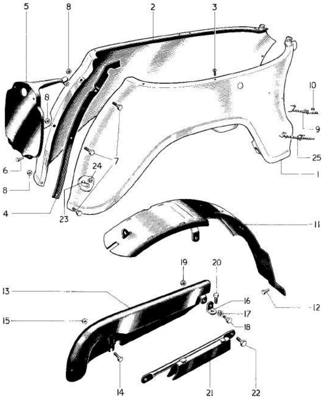
FIG. 14 REAR MUDGUARD, CHAINGUARD AND PANELS
